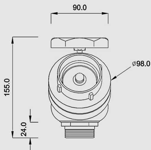
VISTA FRONTAL
